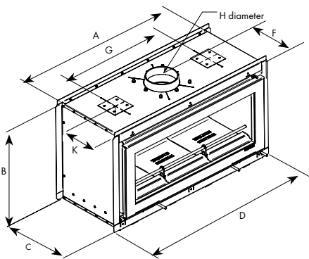
DUPLEX DIMENSIONS
