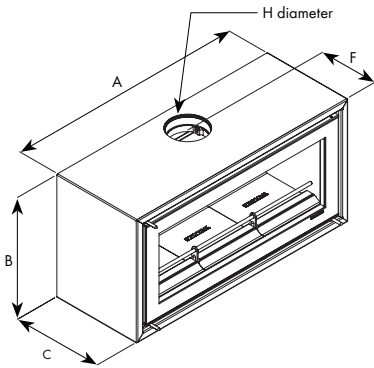
FREESTANDING DIMENSIONS **
