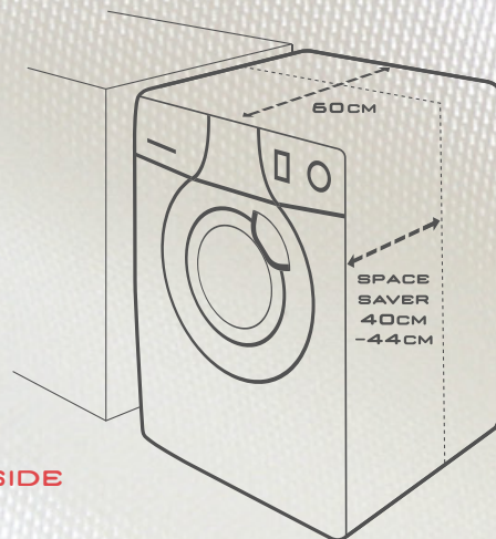
SPACESAVER WASHER DRYER 44 CM DEPTH
