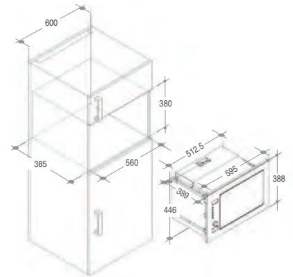
MICG 25 GDFN COMBINATION MICROWAVE OVEN AND GRILL
