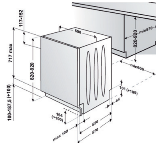
DW600 Aperture cut-out: H820-920 * W600 * D570
